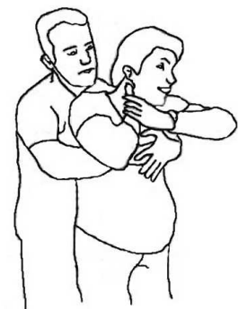
Figure 5.9 : Compressions thoraciques
